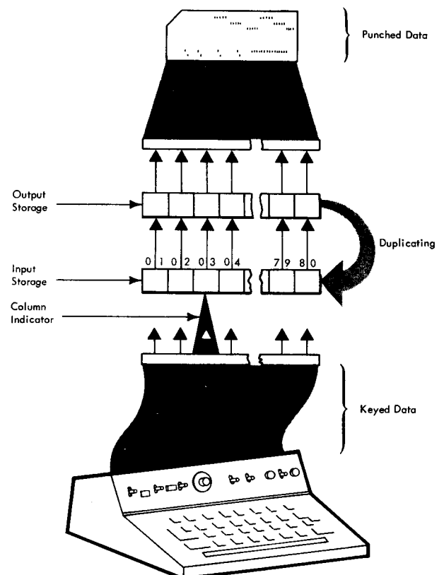
Figure 1. Input and Output Storage
