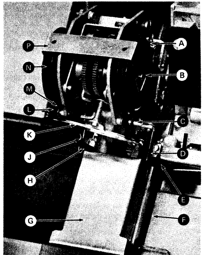
Figure 8. Ribbon Replacement
